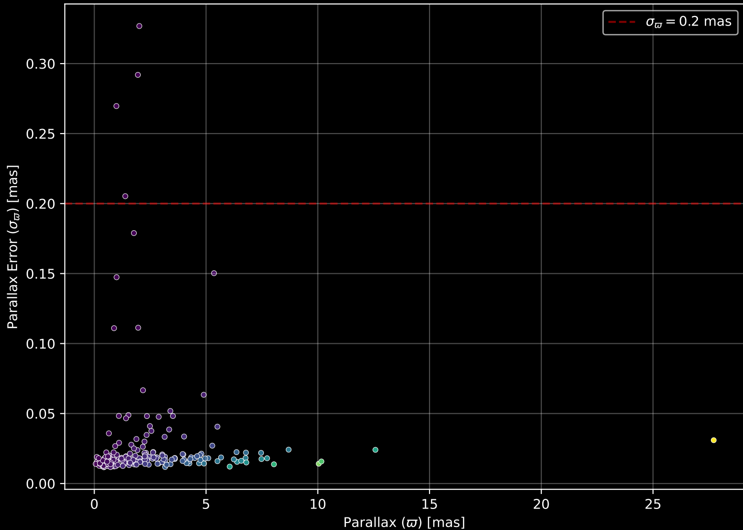
APOGEE DR17 Field: [194+26_MGA] Parallax Quality (n= 203)
