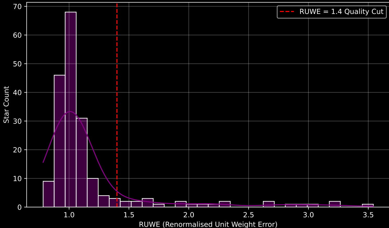
GAPOGEE DR17 Field [194+26_MGA] RUWE Distribution (n= 194)
