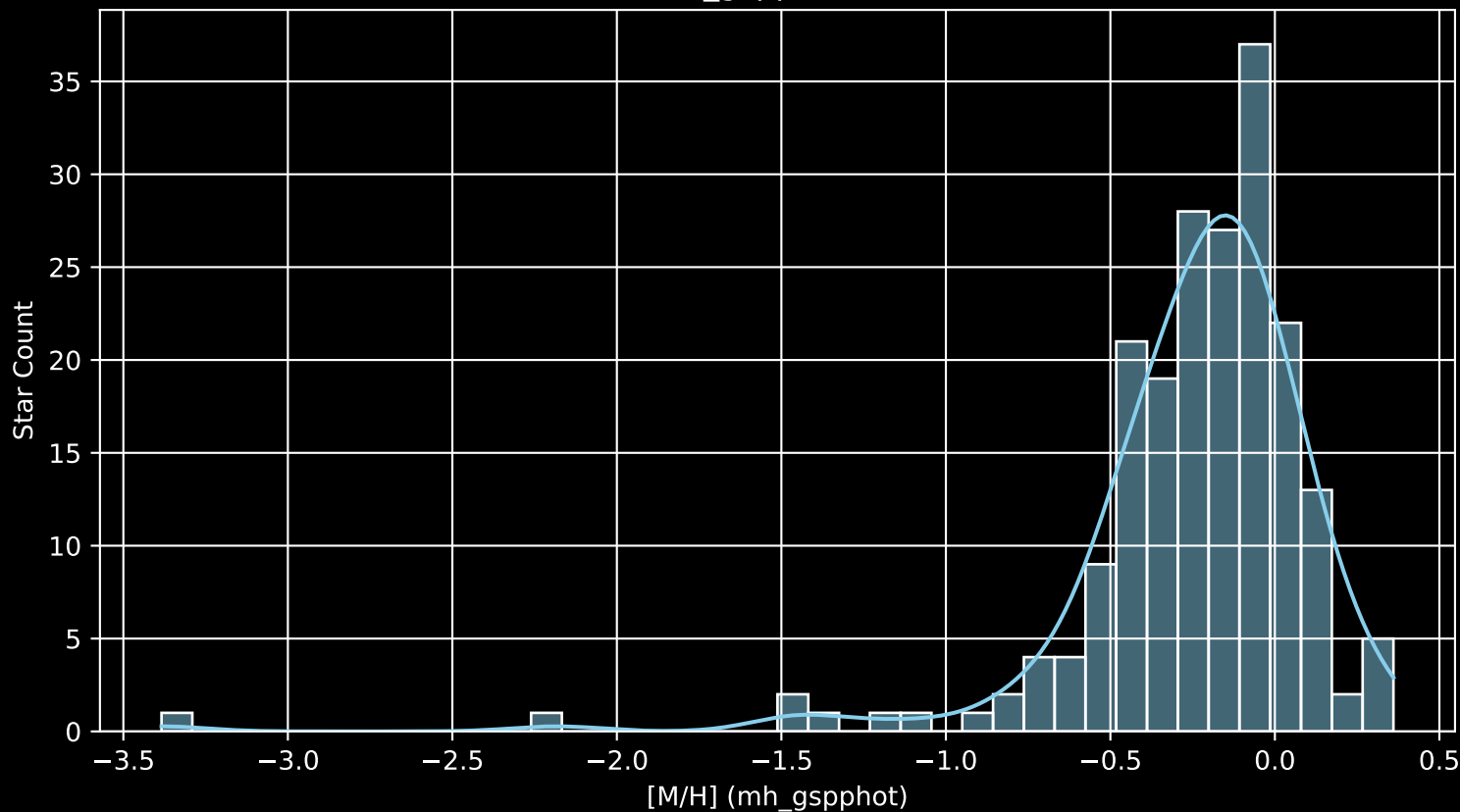
APOGEE DR17 Field: [194+26_MGA [M/H] (mh_gspphot) (n= 201)
