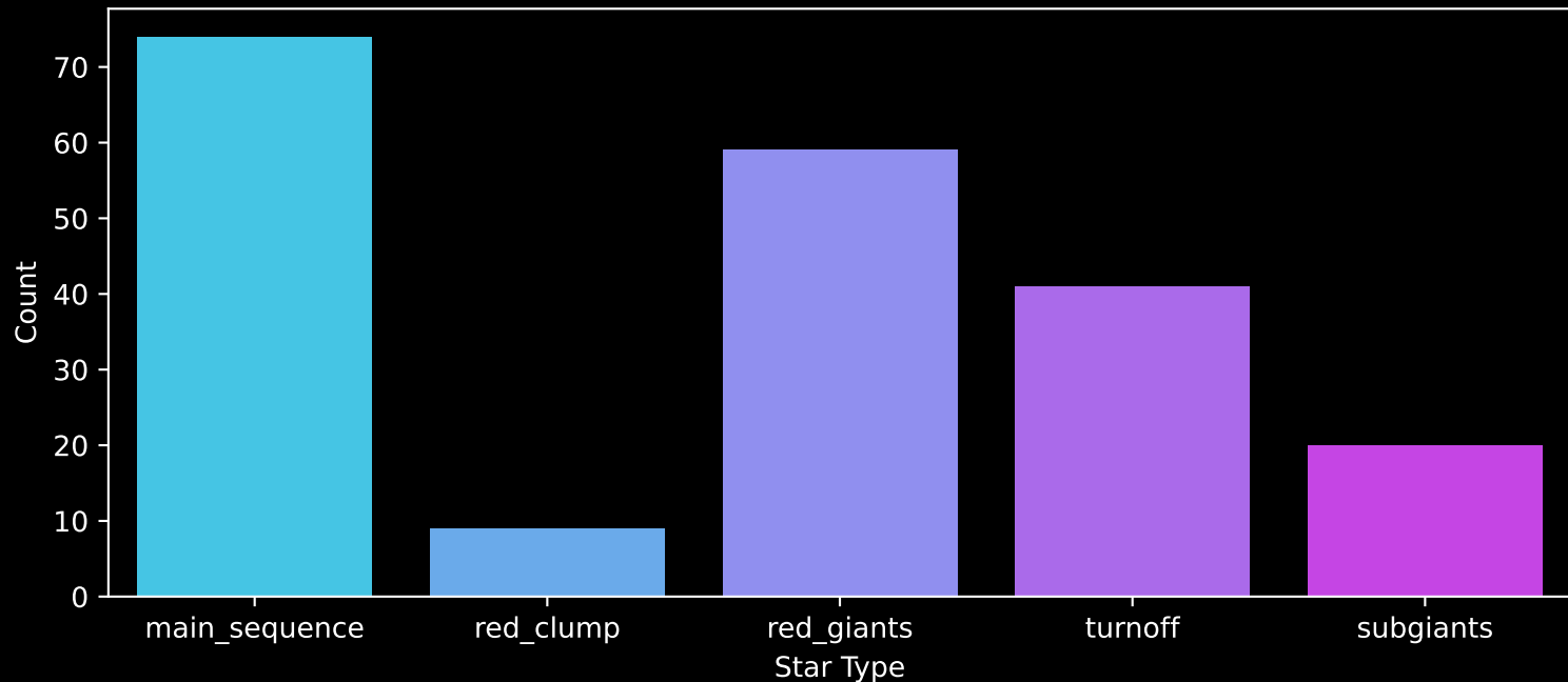
APOGEE DR17 Field: [194+26_MGA] Count plot of Star Type
