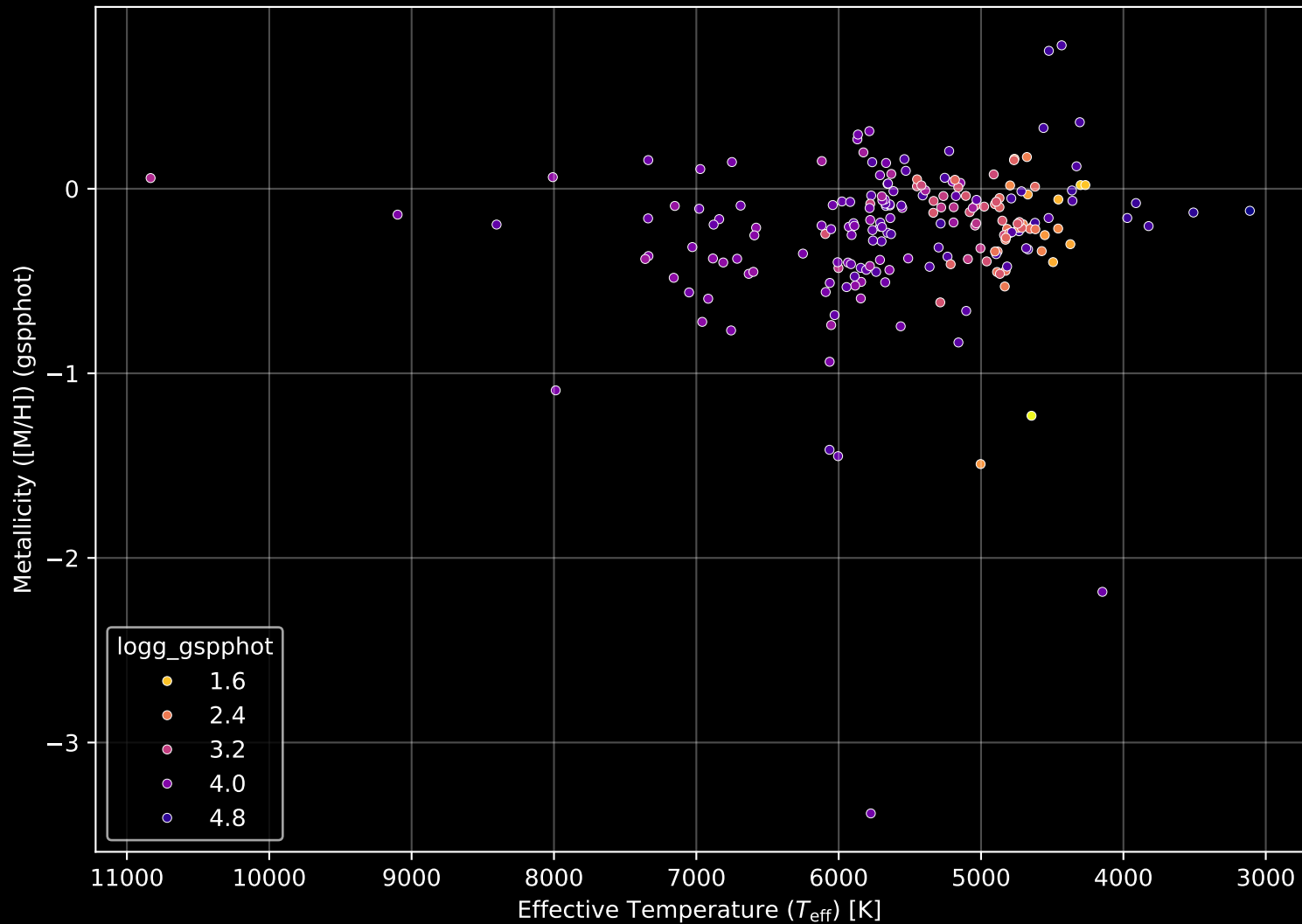
APOGEE DR17 Field: [194+26_MGA] Stellar Population Parameters (n= 203)
