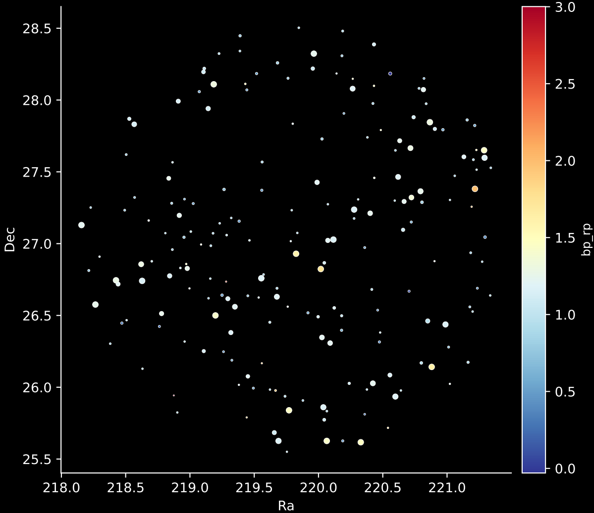
APOGEE DR17 Field: [194+26_MGA] Stars: 203
