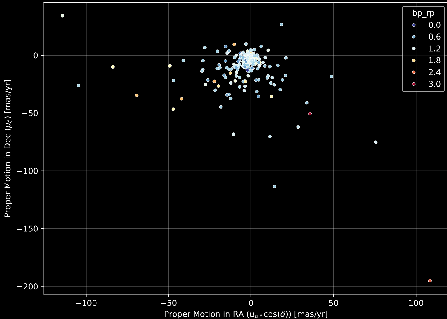
APOGEE DR17 Field: [194+26_MGA] Proper Motion Diagram (n= 203)
